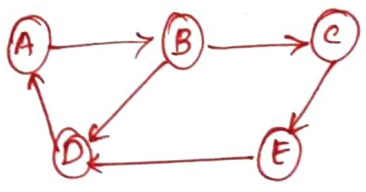
Directed graph
