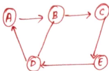
Directed graph
