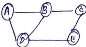
undirected graph
