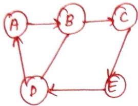
Directed graph.
