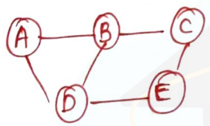
Undirected graph
